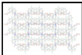
Fig. 4. Unit-cell contents for (I) viewed in projection down the c axis showing the stacking of the layers, illustrated in Fig. 3, along the a direction with the C–H···Cl contacts shown as pink dashed lines. Colour code as for Fig. 2.
